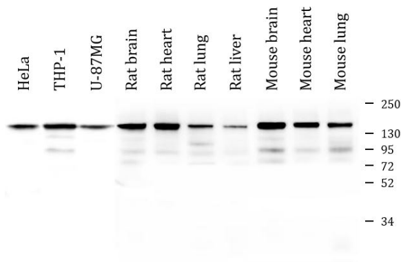
ARG43090 anti-BAG6 / BAT3 antibody WB image Western blot: 50 µg of sample under reducing conditions. HeLa, THP-1, U-87MG, Rat brain, Rat heart, Rat lung, Rat liver, Mouse brain, Mouse heart and Mouse lung lysates stained with ARG43090 anti-BAG6 / BAT3 antibody at 0.5 µg/ml dilution, overnight at 4°C.
