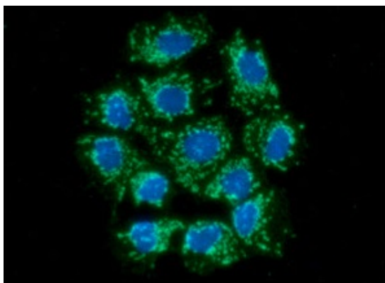
ARG57162 anti-AIF antibody [22E9] ICC/IF image
