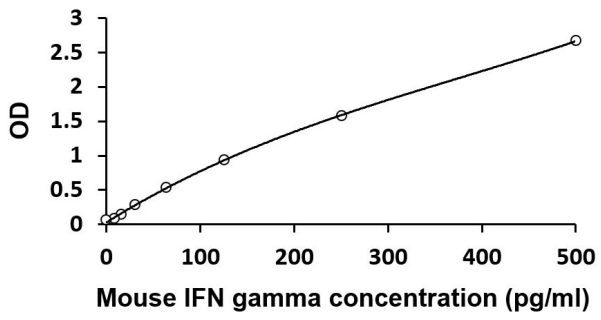
ARG80205 Mouse IFN gamma ELISA Kit standard curve image
