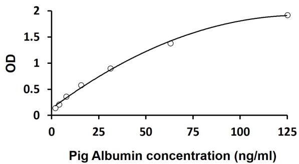
ARG81166 Pig Albumin ELISA Kit standard curve image
