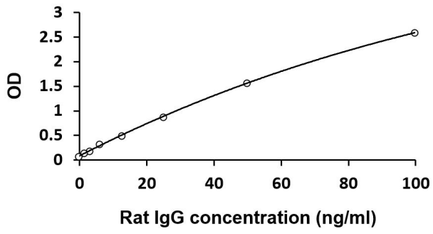
ARG81184 Rat IgG ELISA Kit standard curve image
