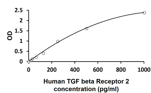
ARG81882 Human TGF beta Receptor 2 ELISA Kit standard curve image ARG81882 Human TGF beta Receptor 2 ELISA Kit results of a typical standard run with optical density reading at 450 nm.
